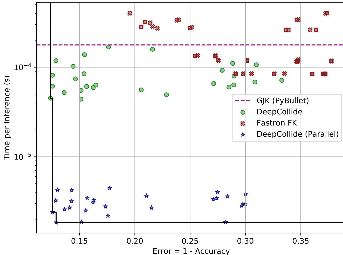
Error = (1 - Accuracy) vs. Time per Inference (s): 21 DoF, 30K Train, 5K Test
